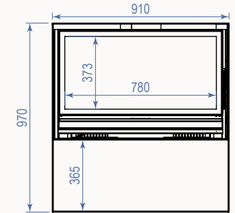
VENTILART PRO 90 DF/DK WOODBOX (Base Nordic Pro)
