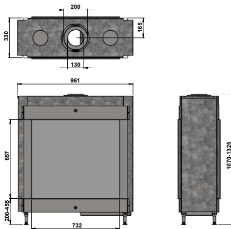
Trimline 73H Tunnel
