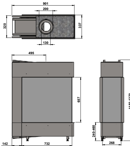
Trimline 73 Room Divider
